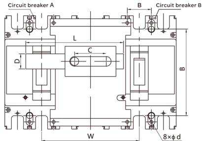
Fig 6 Mechanical interlock dimension diagram
