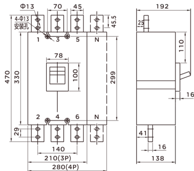
Fig 12 RDM1-125M circuit breaker overall and installation dimension
