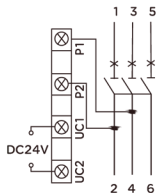
Fig 1 DC 24V connection diagram
