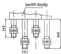
RDM1-63, 125, 250 back connection
