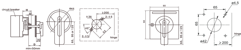
Round extension rotary handle hole size diagram
