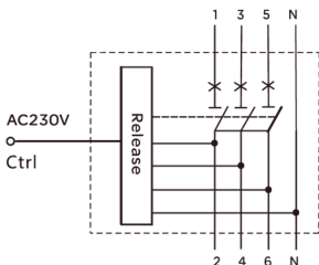
Special circuit breaker for pre-paid meter diagram
