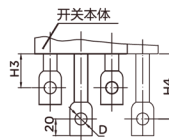
RDM1-400, 630, 800 back connection
