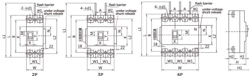
Fig 7 RDM1-63-800 Front connection overall and installation dimension
